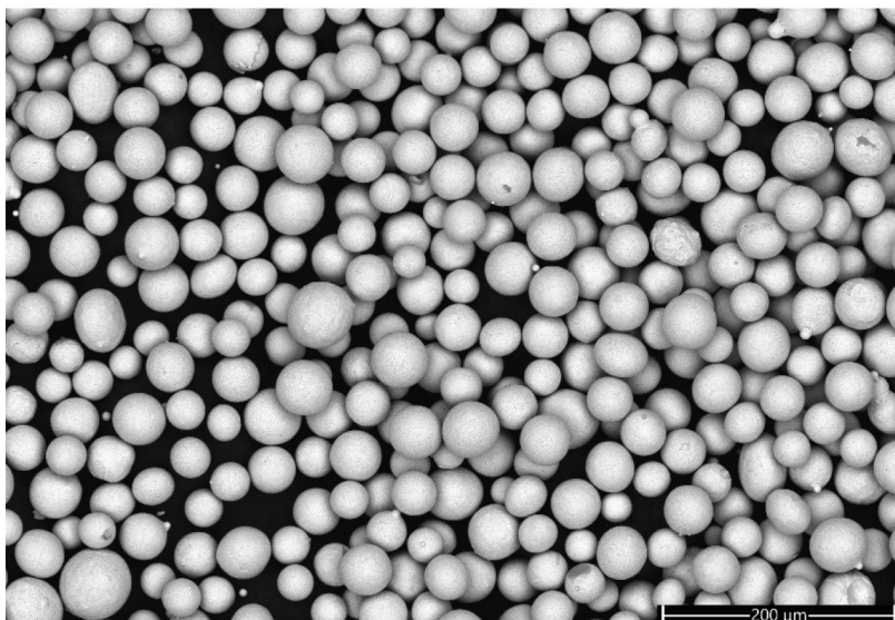
Typical morphology of L-PBF size powder
