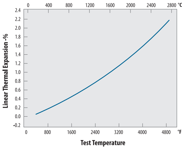
Thermal Expansion versus Temperature
