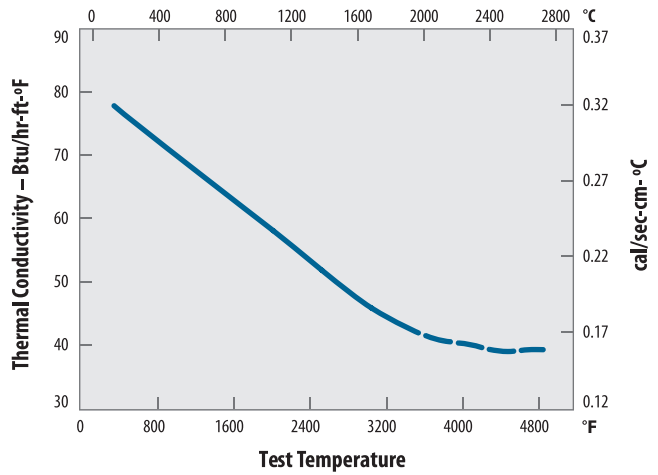
Thermal Conductivity versus Temperature
