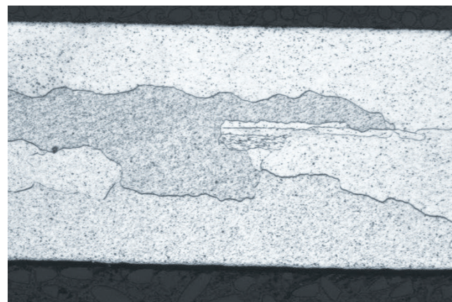
Transverse direction
